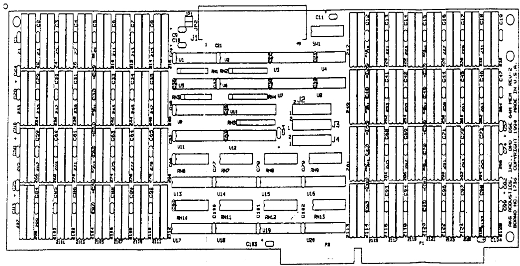
Figure 4: 64MB Zip Memory Board (32MB Zip boards are similar, but chip sockets are half populated)
